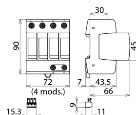
Dimensions DG MP TNS 275 FM
