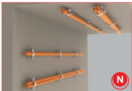
Attache OMEGA E90 – p. 137
